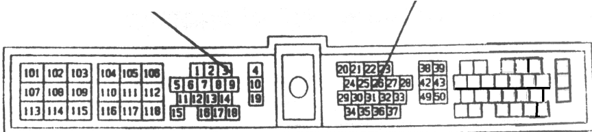
(Wire side of plug)
